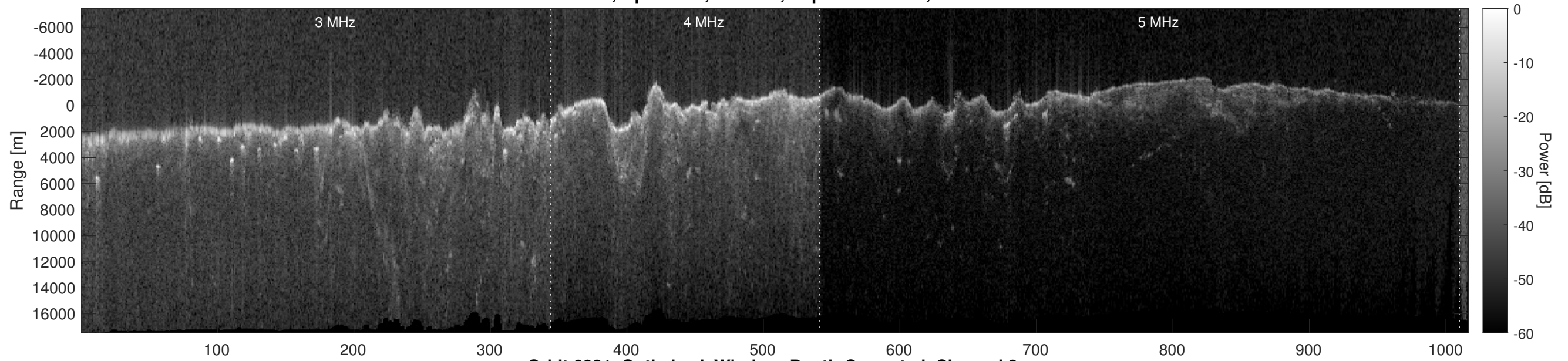
Orbit 6821, Optimized, Window, Depth-Corrected, Channel 2
