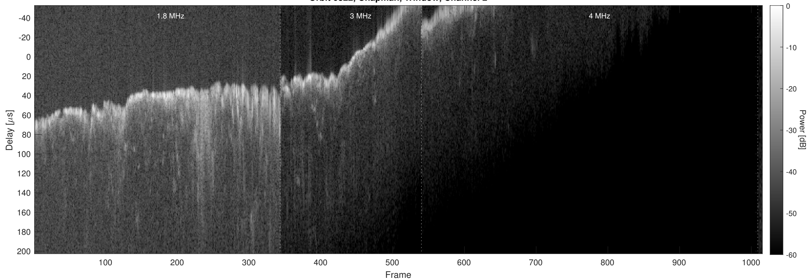
Orbit 6822, Chapman, Window, Channel 2
