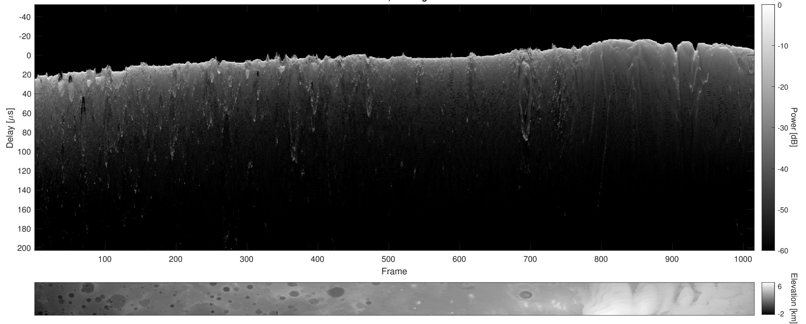
Orbit 6822, Cluttergram
