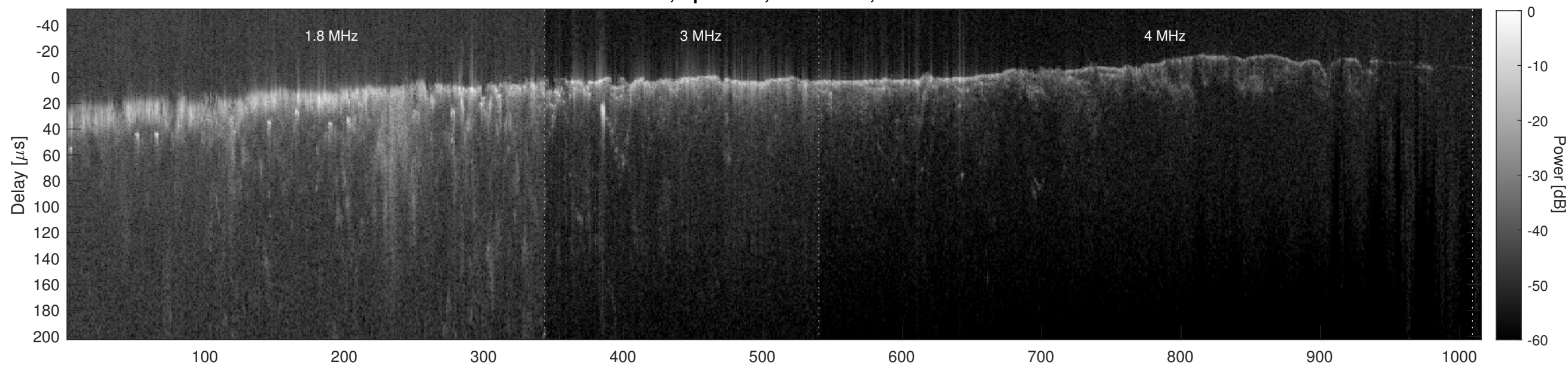
Orbit 6822, Cluttergram
