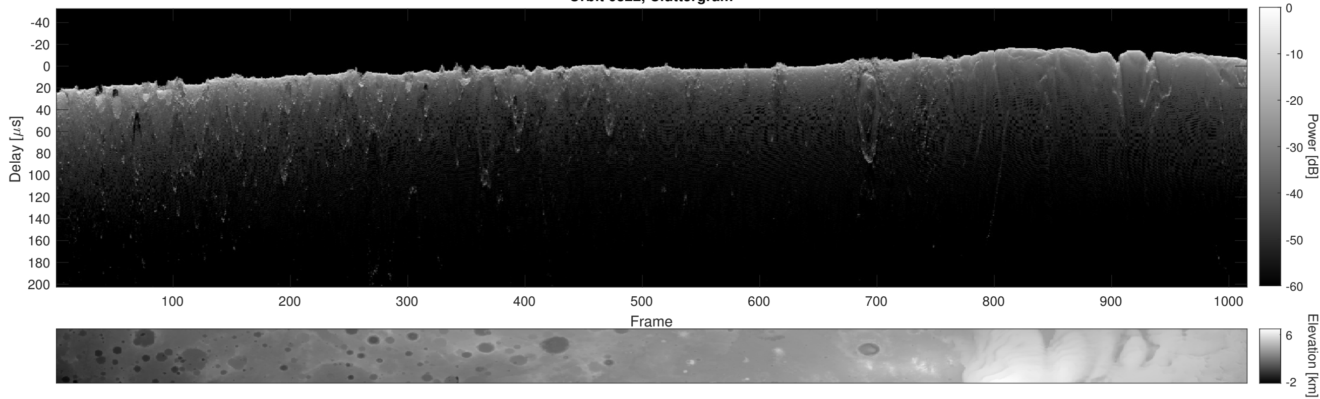
Orbit 6822, Cluttergram
