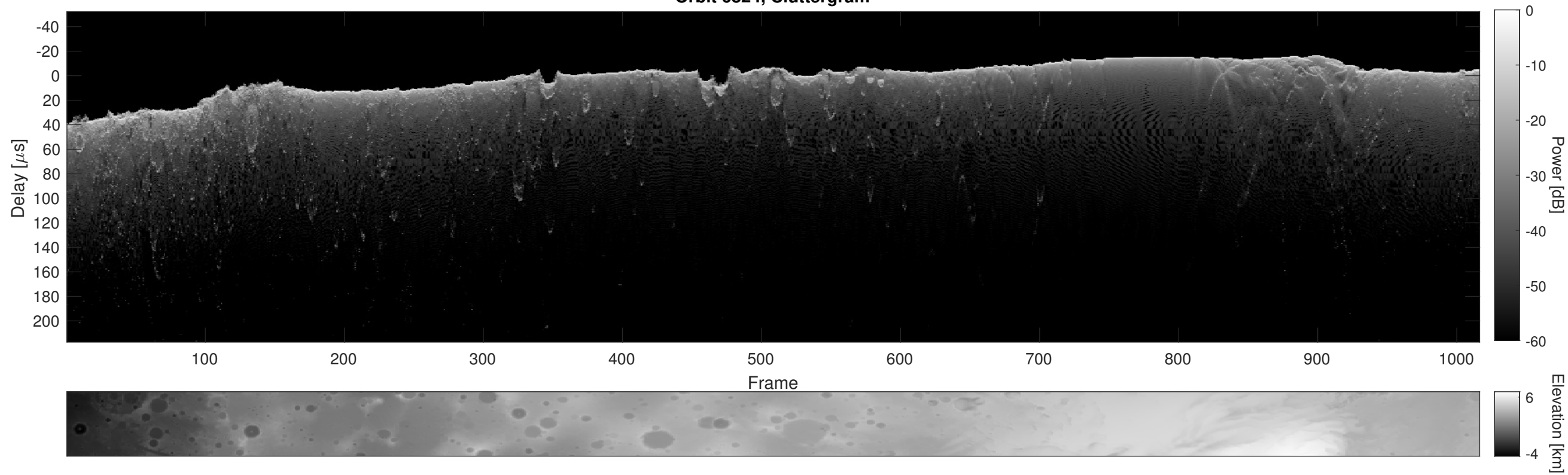
Orbit 6824, Cluttergram
