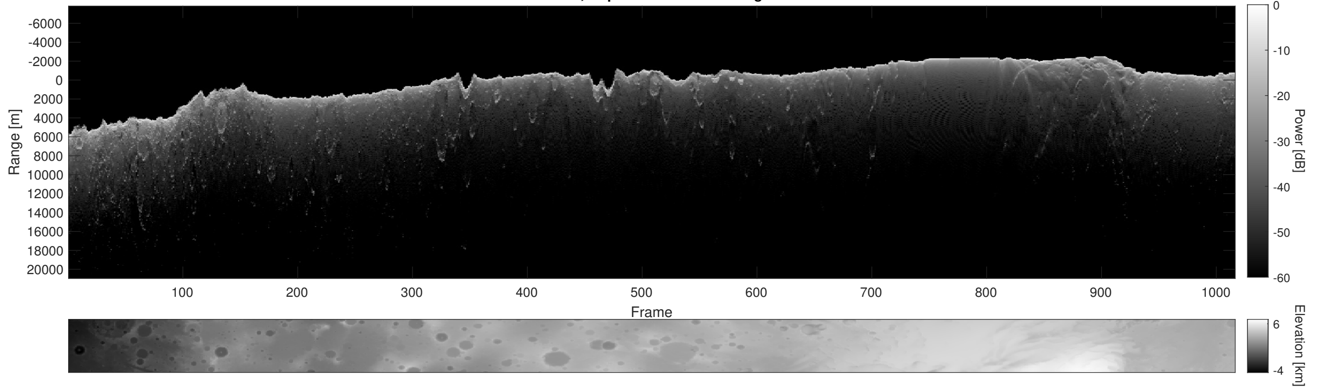
Orbit 6824, Depth-Corrected Cluttergram
