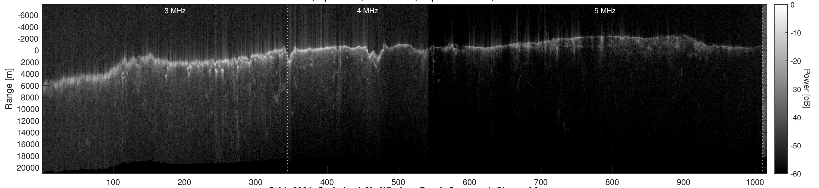
Orbit 6824, Optimized, No Window, Depth-Corrected, Channel 2
