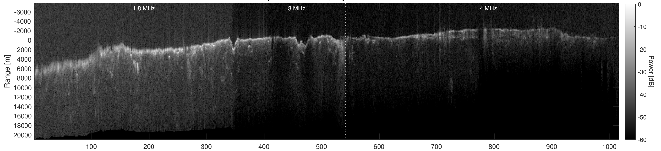
Orbit 6824, Depth-Corrected Cluttergram
