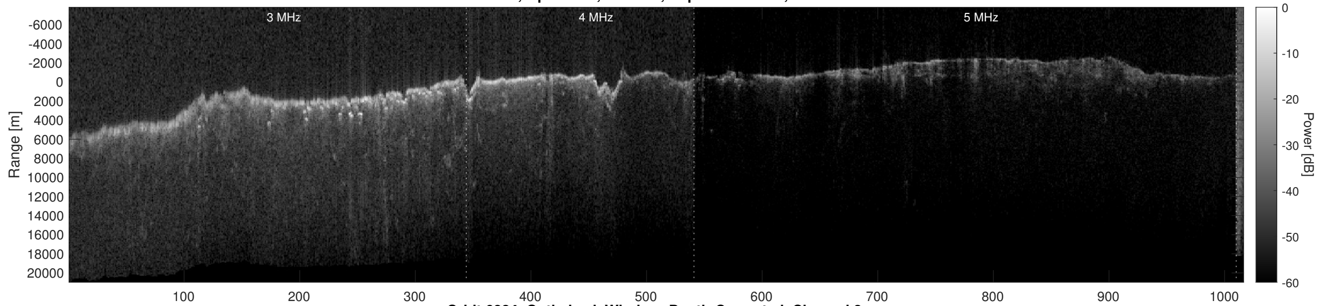
Orbit 6824, Optimized, Window, Depth-Corrected, Channel 2
