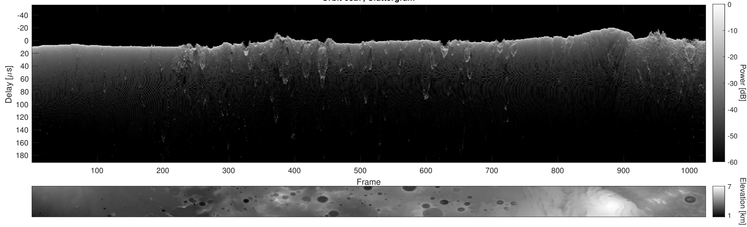
Orbit 6827, Cluttergram
