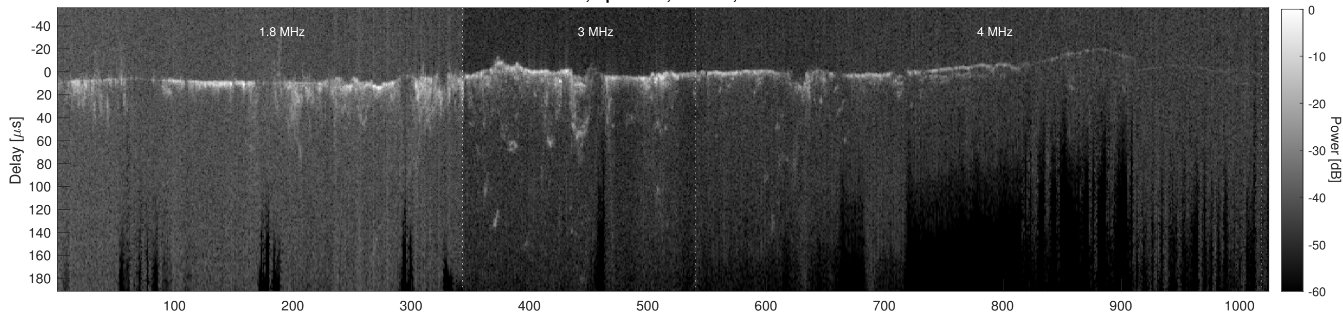
Orbit 6827, Cluttergram
