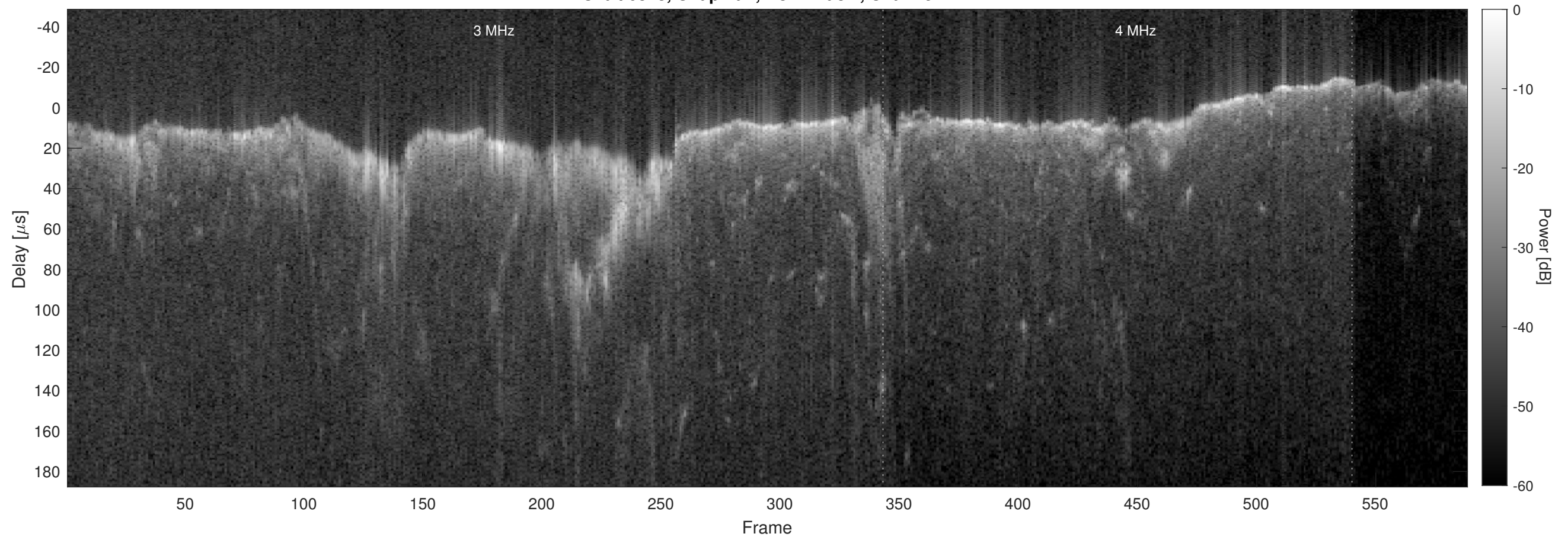
Orbit 6828, Chapman, No Window, Channel 2
