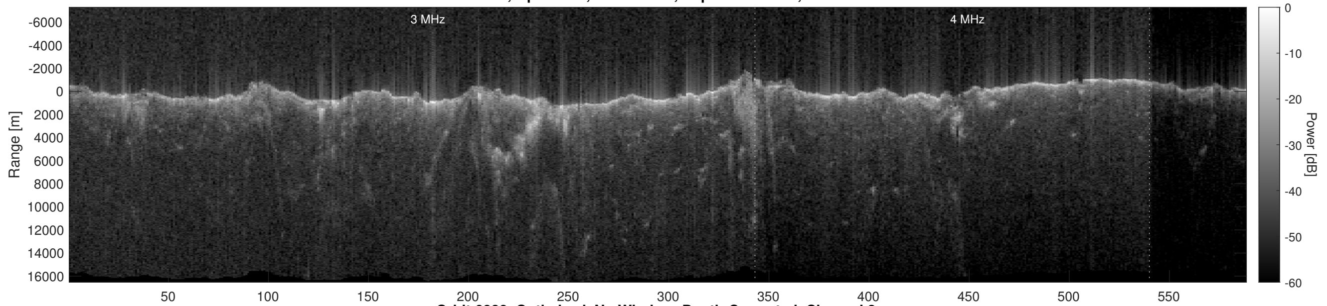
Orbit 6828, Optimized, No Window, Depth-Corrected, Channel 2
