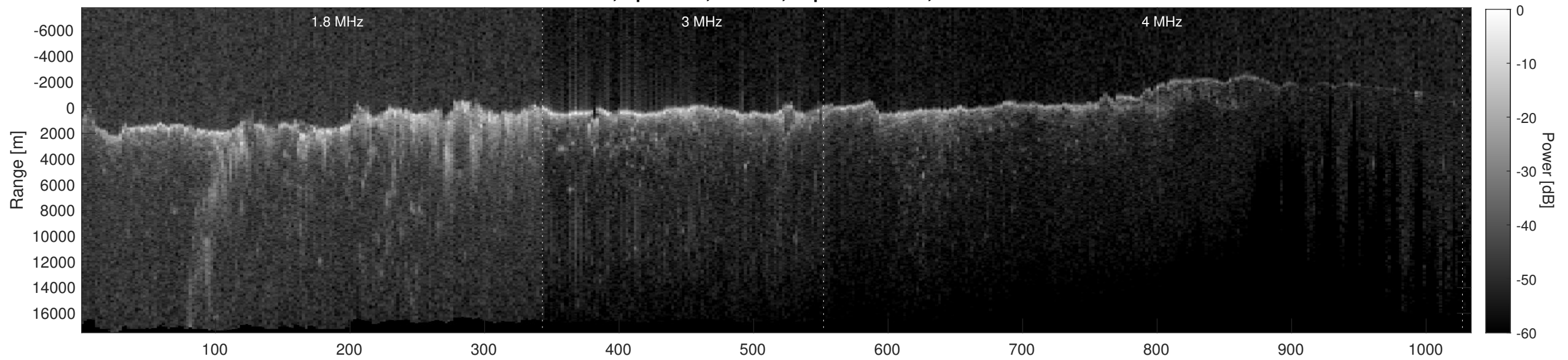
Orbit 6829, Depth-Corrected Cluttergram
