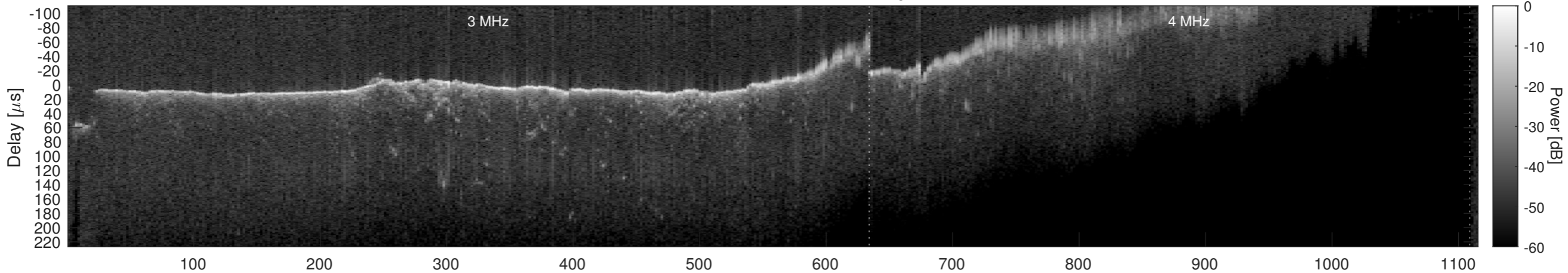
Orbit 6830, Window, Channel 2, Optimized
