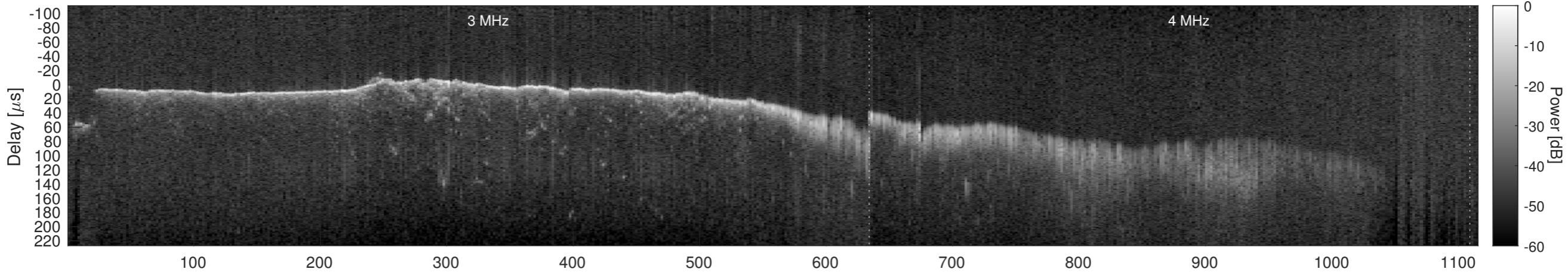
Orbit 6830, Window, Channel 2, Chapman
