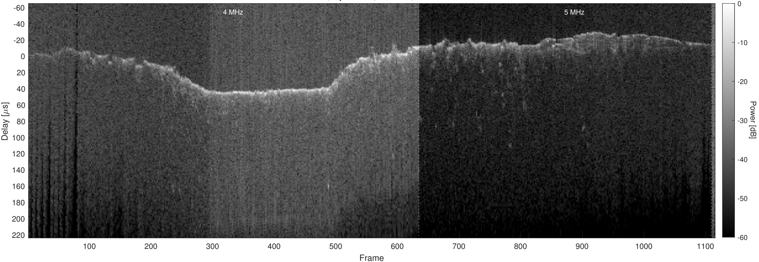
Orbit 6832, Optimized, Window, Channel 2
