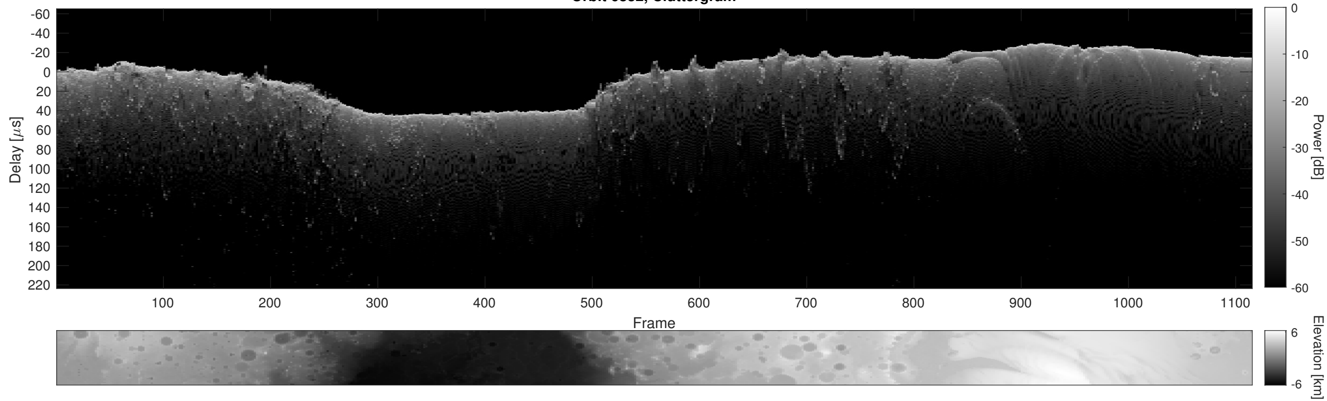
Orbit 6832, Cluttergram
