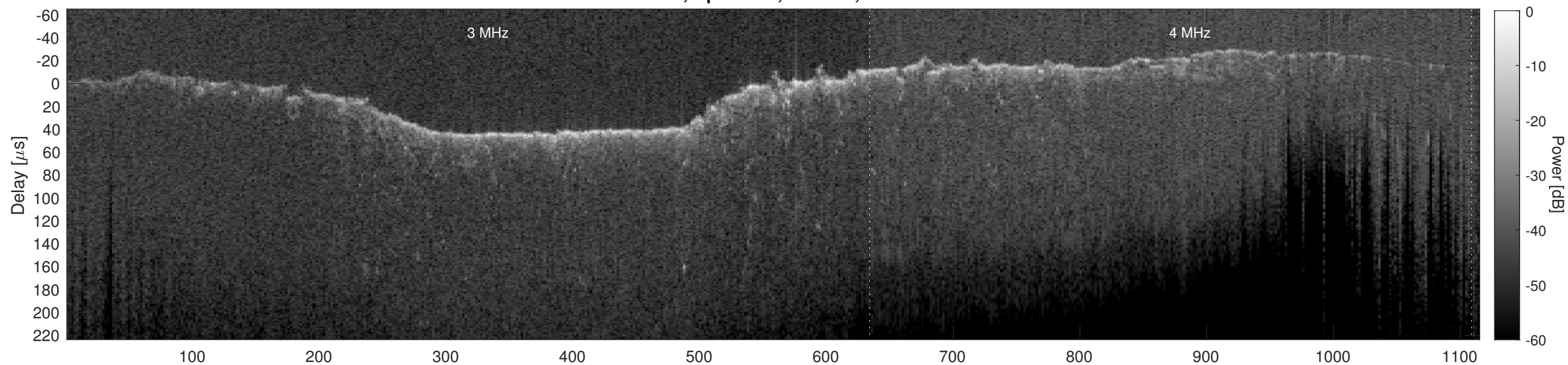
Orbit 6832, Cluttergram
