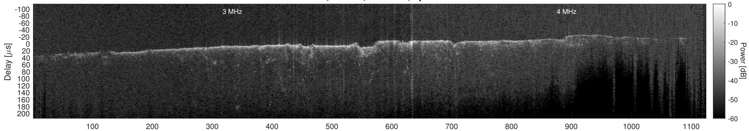
Orbit 6833, Cluttergram
