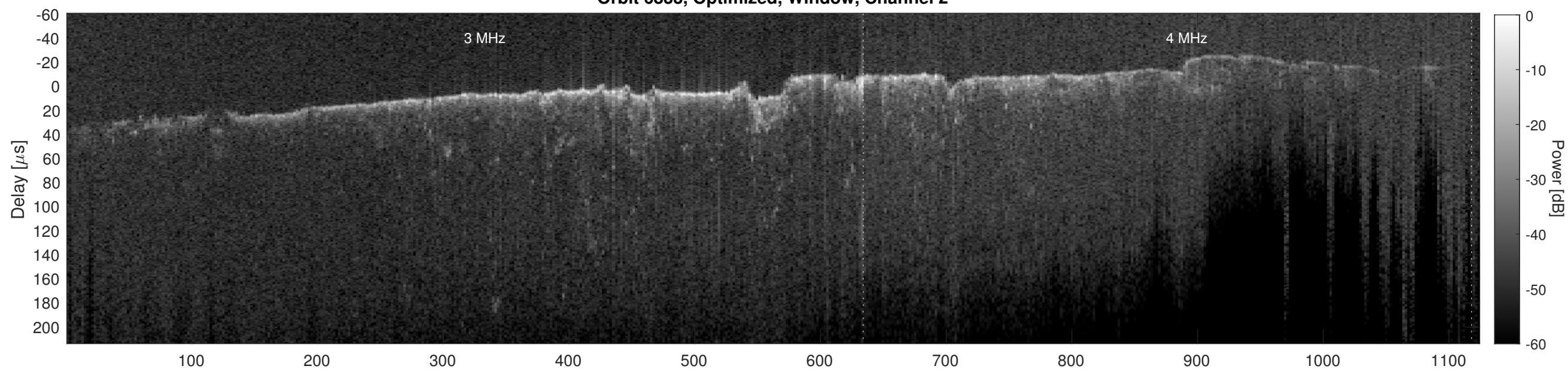
Orbit 6833, Cluttergram
