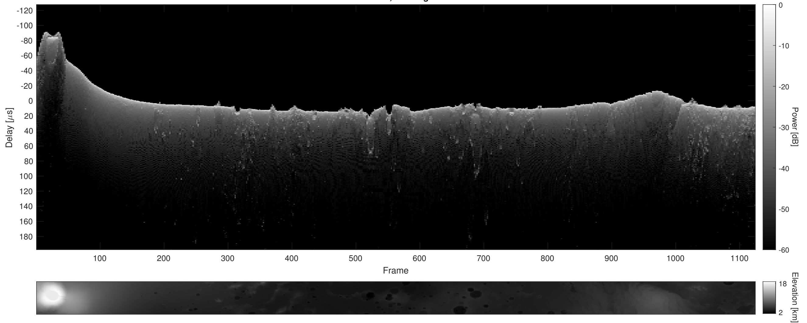
Orbit 6834, Cluttergram
