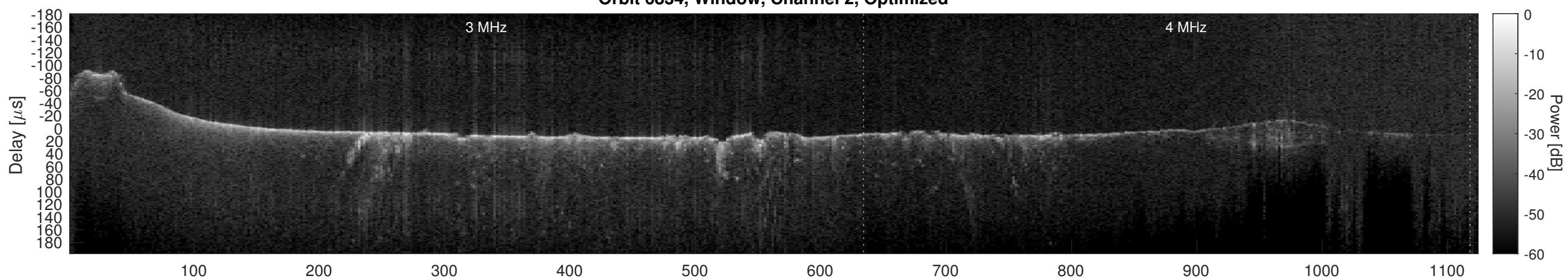
Orbit 6834, Cluttergram
