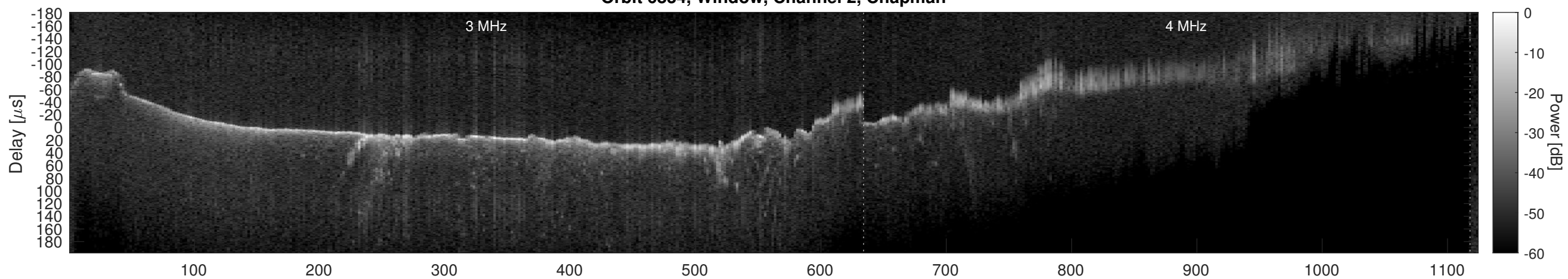
Orbit 6834, Window, Channel 2, Optimized
