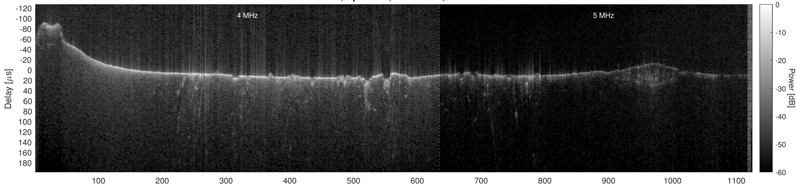
Orbit 6834, Optimized, No Window, Channel 2
