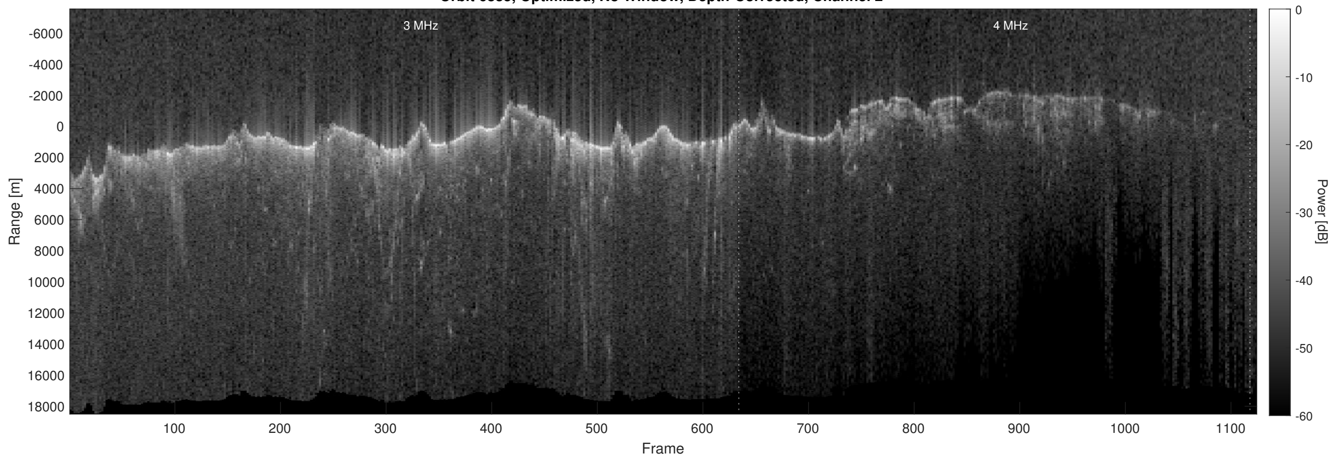
Orbit 6835, Optimized, No Window, Depth-Corrected, Channel 2
