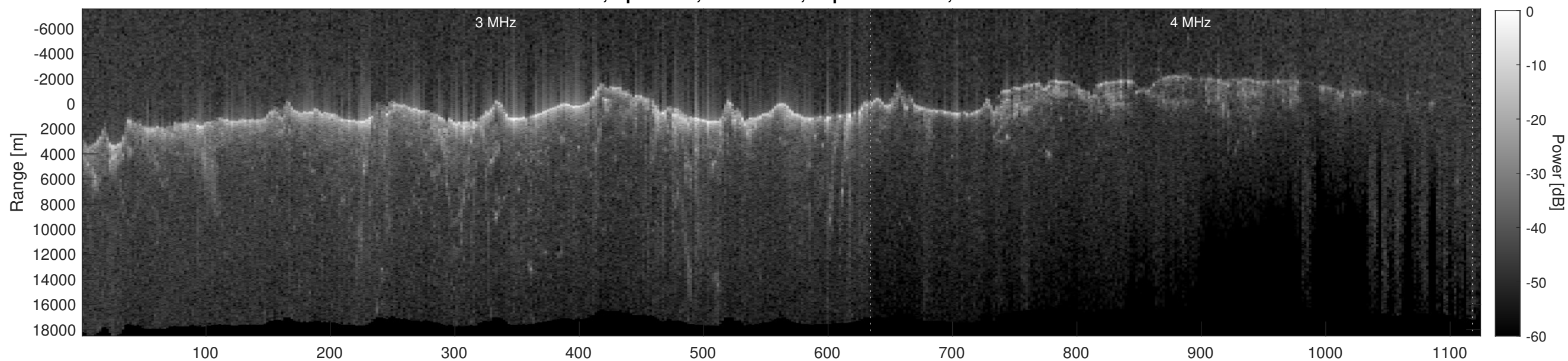
Orbit 6835, Depth-Corrected Cluttergram
