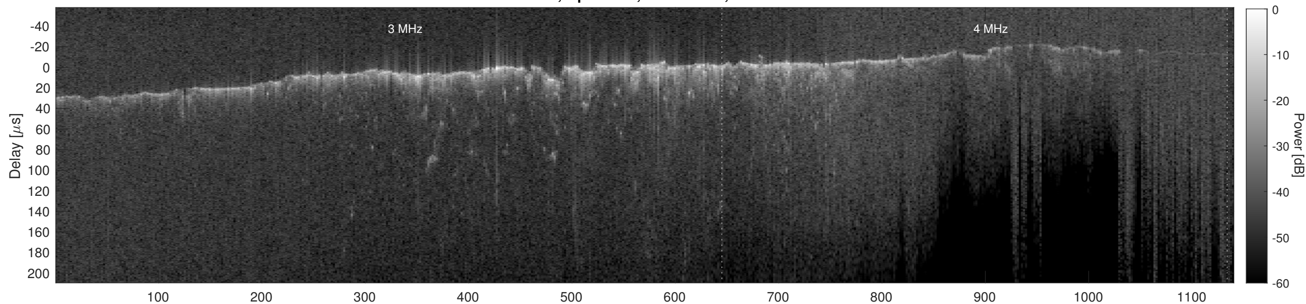
Orbit 6840, Cluttergram
