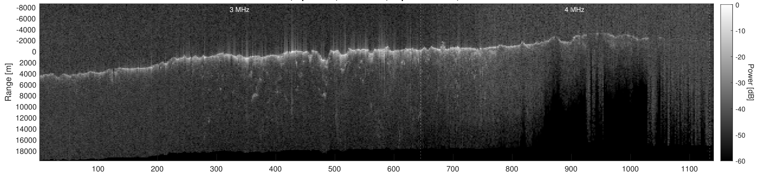
Orbit 6840, Depth-Corrected Cluttergram
