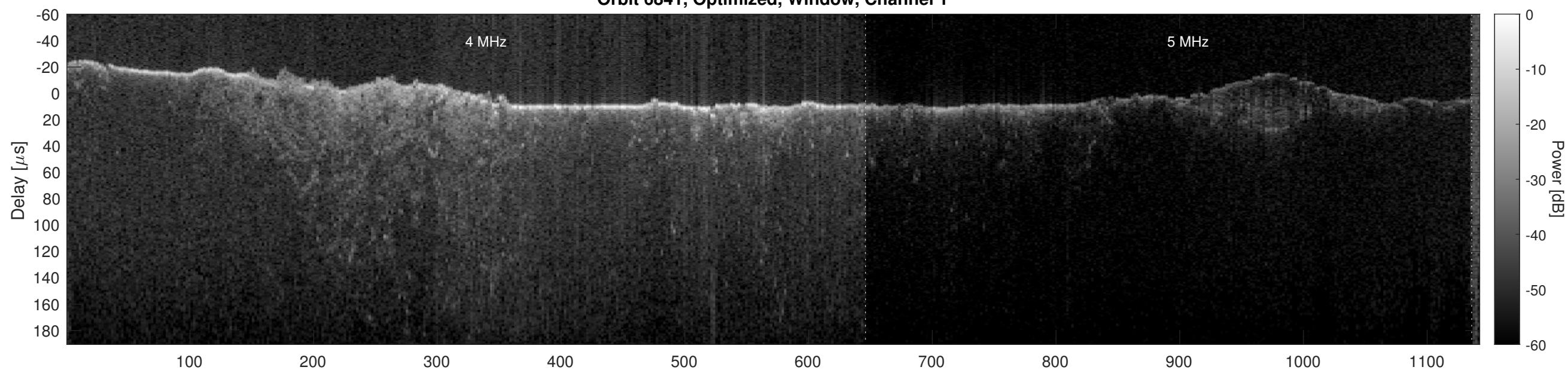
Orbit 6841, Optimized, Window, Channel 2
