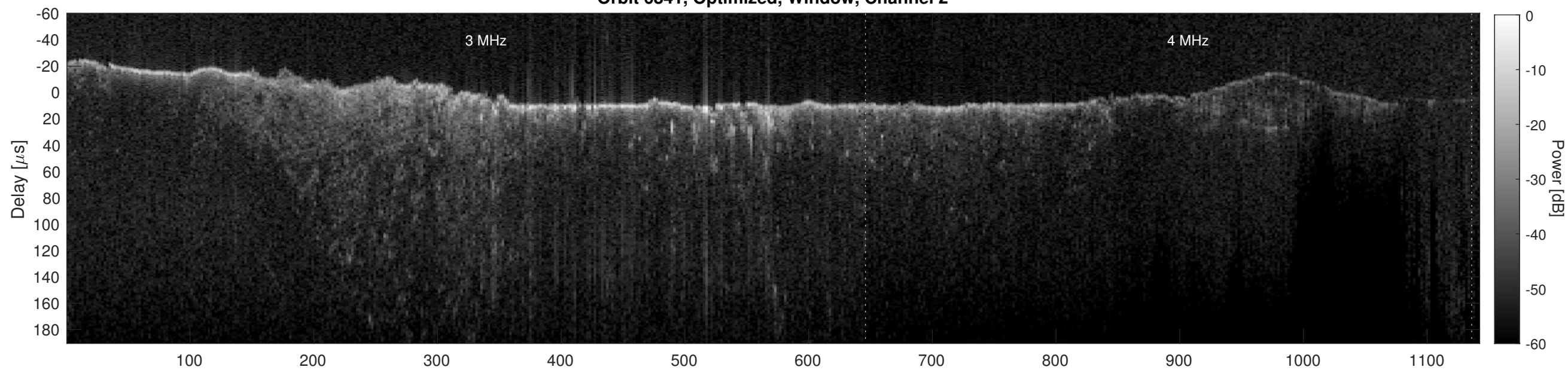
Orbit 6841, Cluttergram
