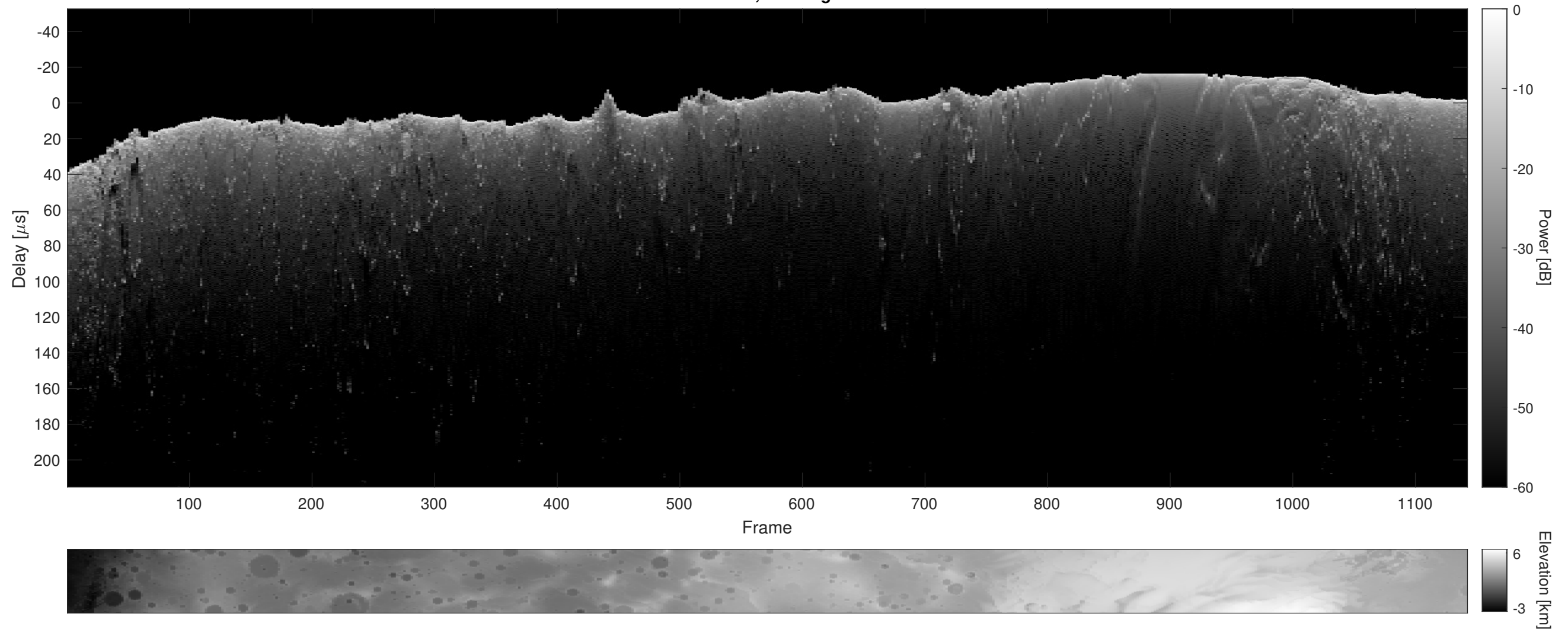
Orbit 6842, Cluttergram
