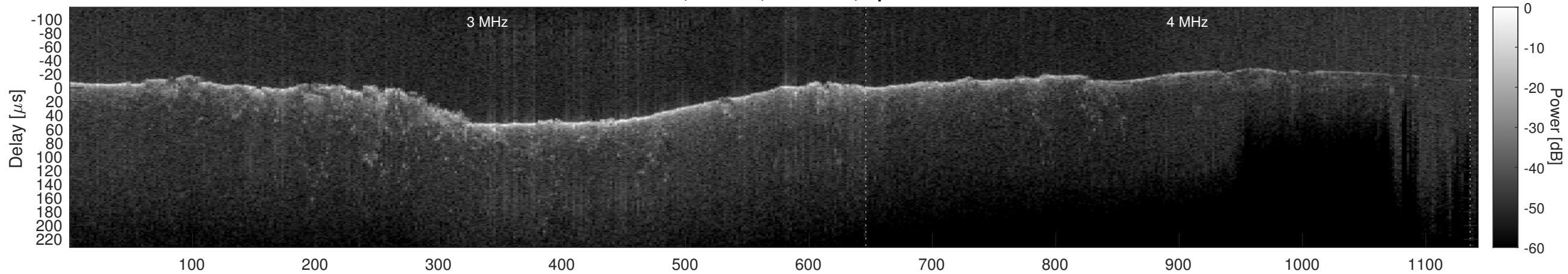
Orbit 6843, Cluttergram
