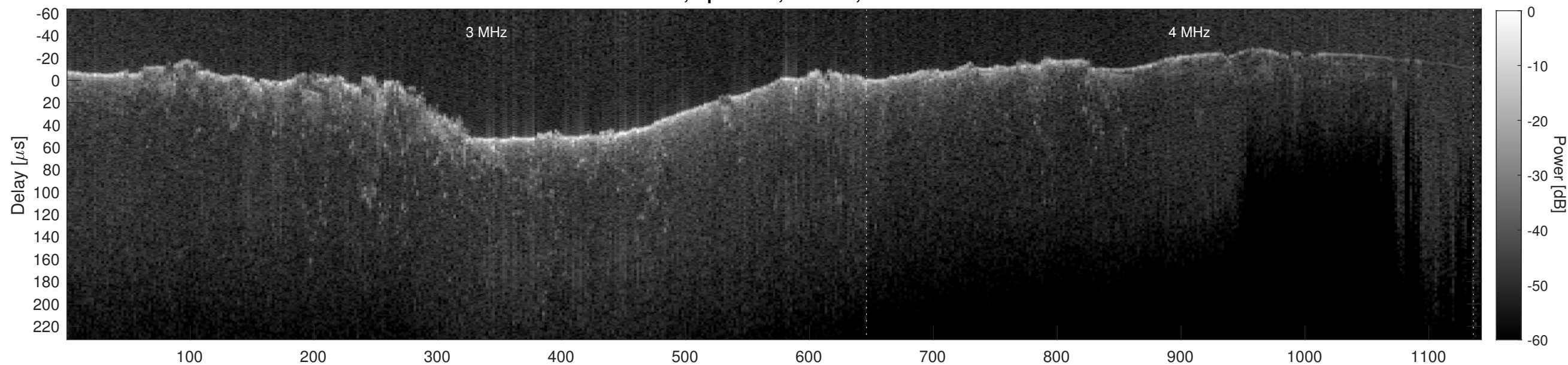
Orbit 6843, Cluttergram
