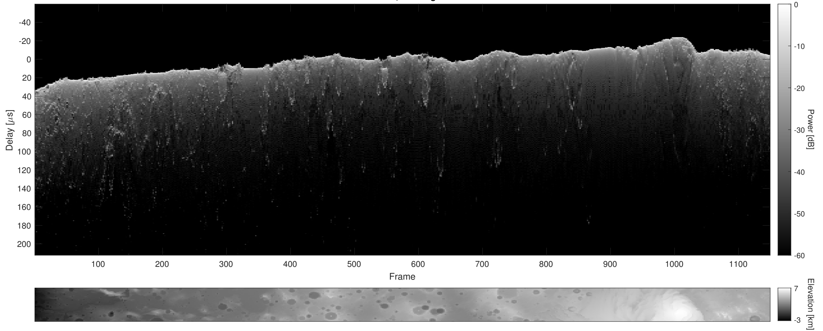
Orbit 6845, Cluttergram
