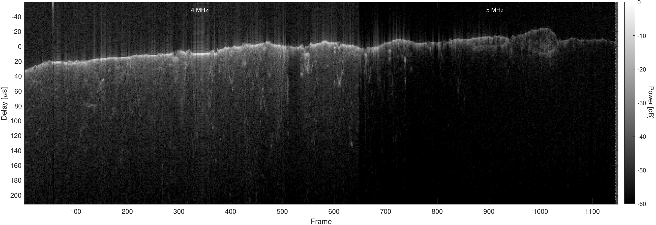
Orbit 6845, Optimized, No Window, Channel 2
