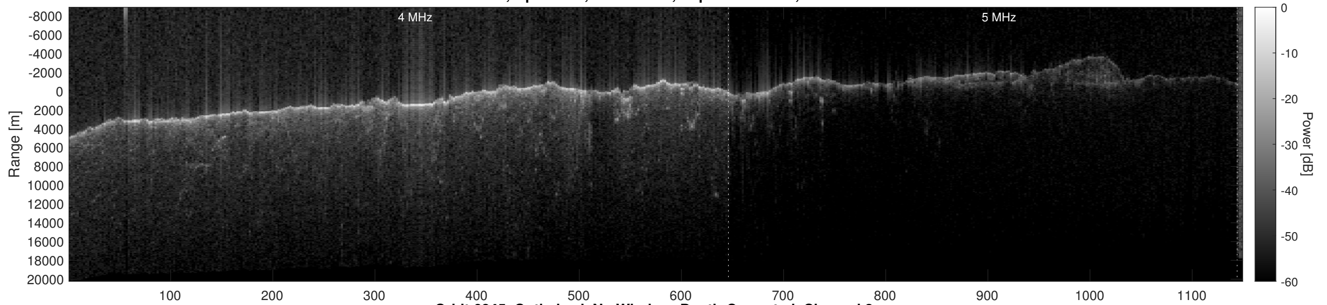
Orbit 6845, Optimized, No Window, Depth-Corrected, Channel 2
