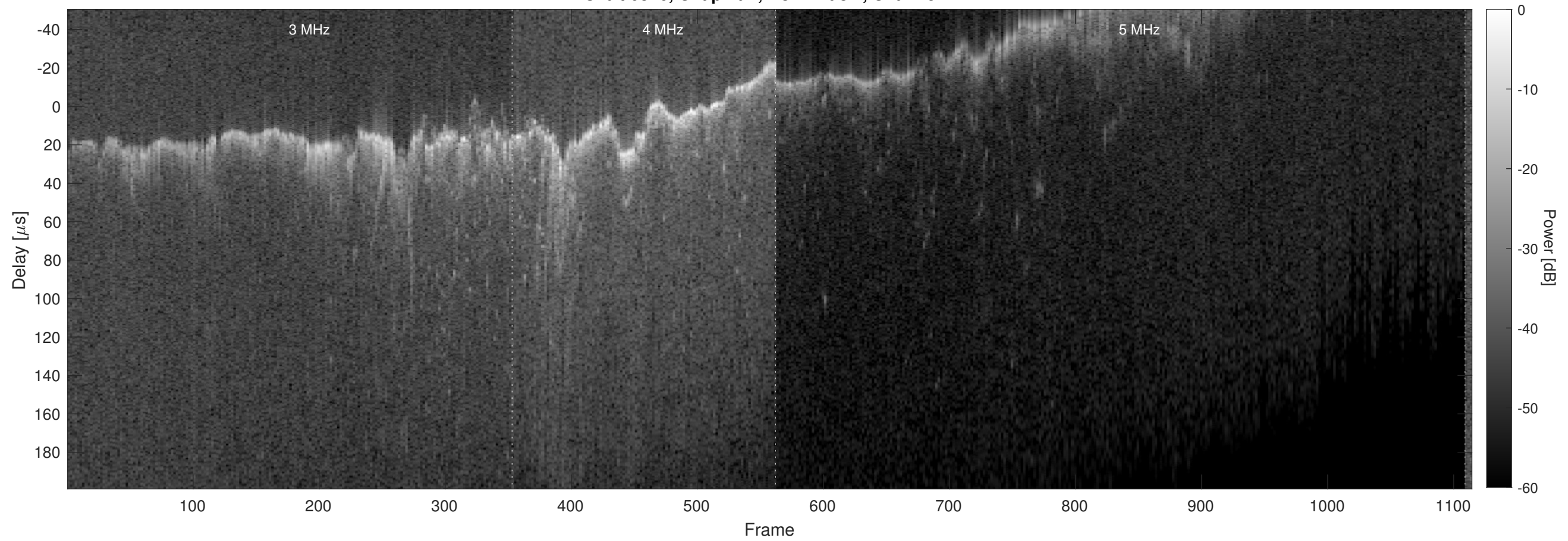
Orbit 6846, Chapman, No Window, Channel 2
