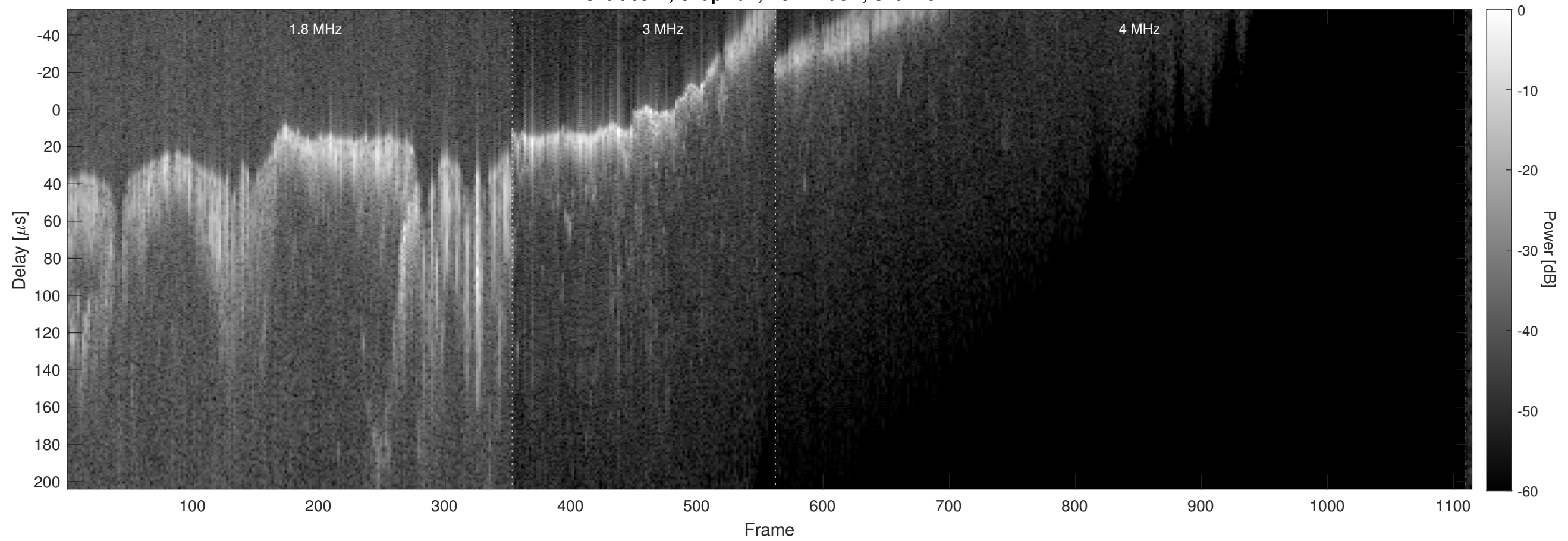
Orbit 6847, Chapman, No Window, Channel 2
