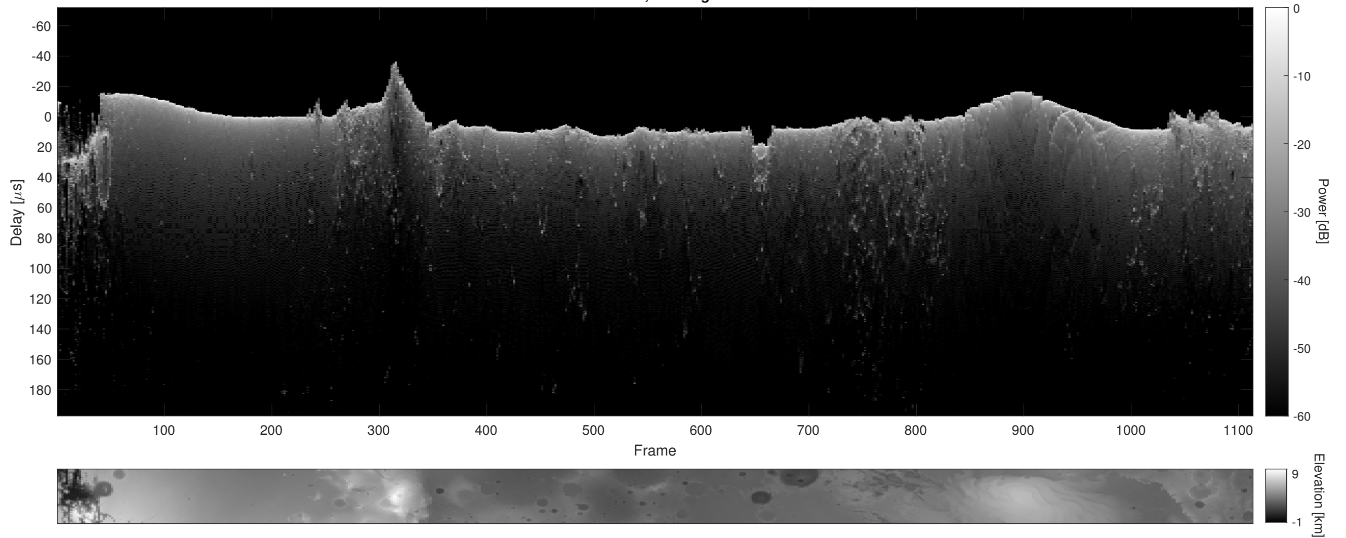
Orbit 6848, Cluttergram
