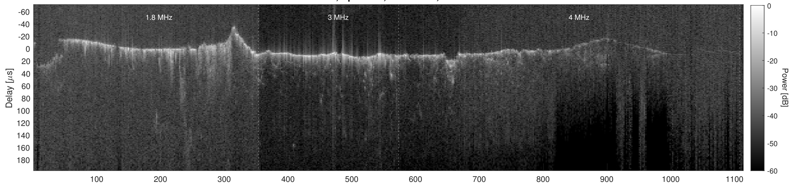
Orbit 6848, Cluttergram
