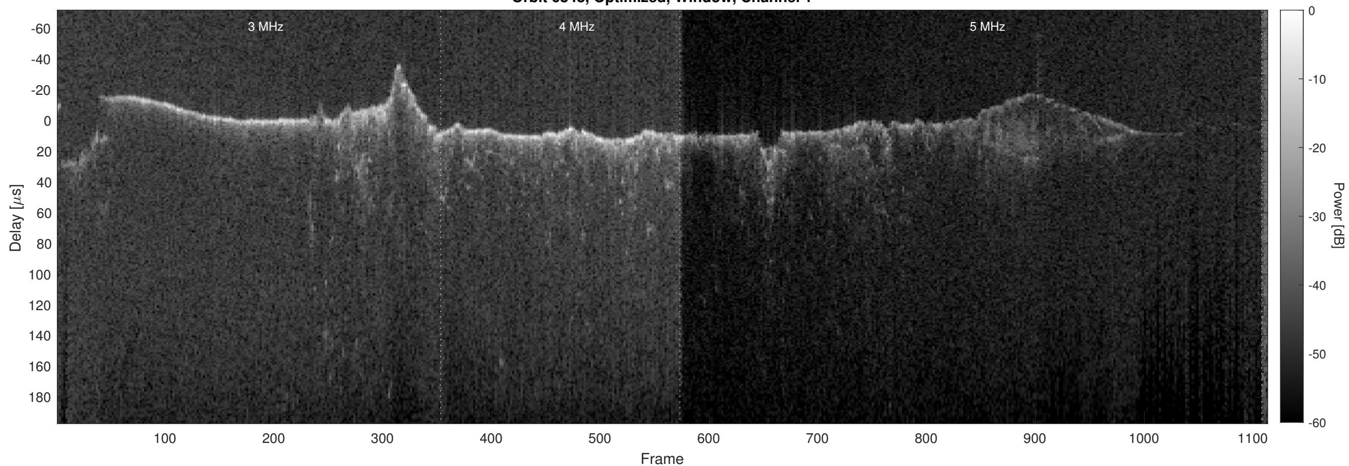
Orbit 6848, Optimized, Window, Channel 2
