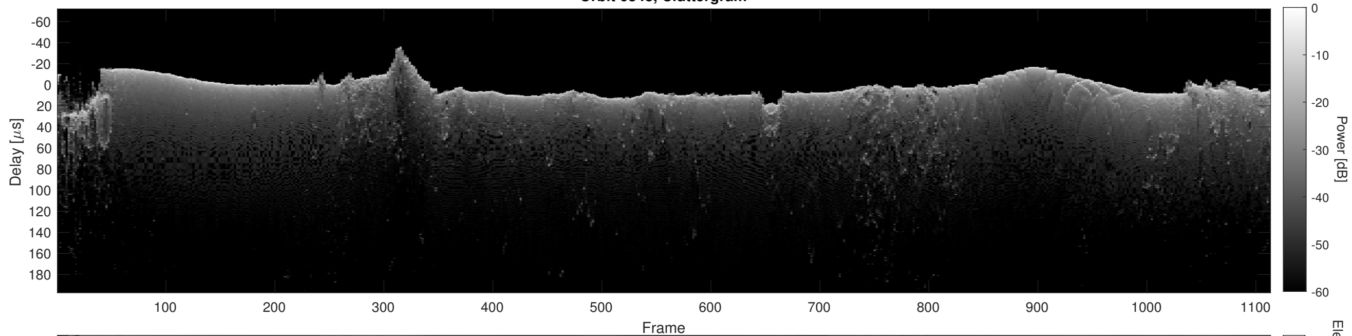
Orbit 6848, Cluttergram
