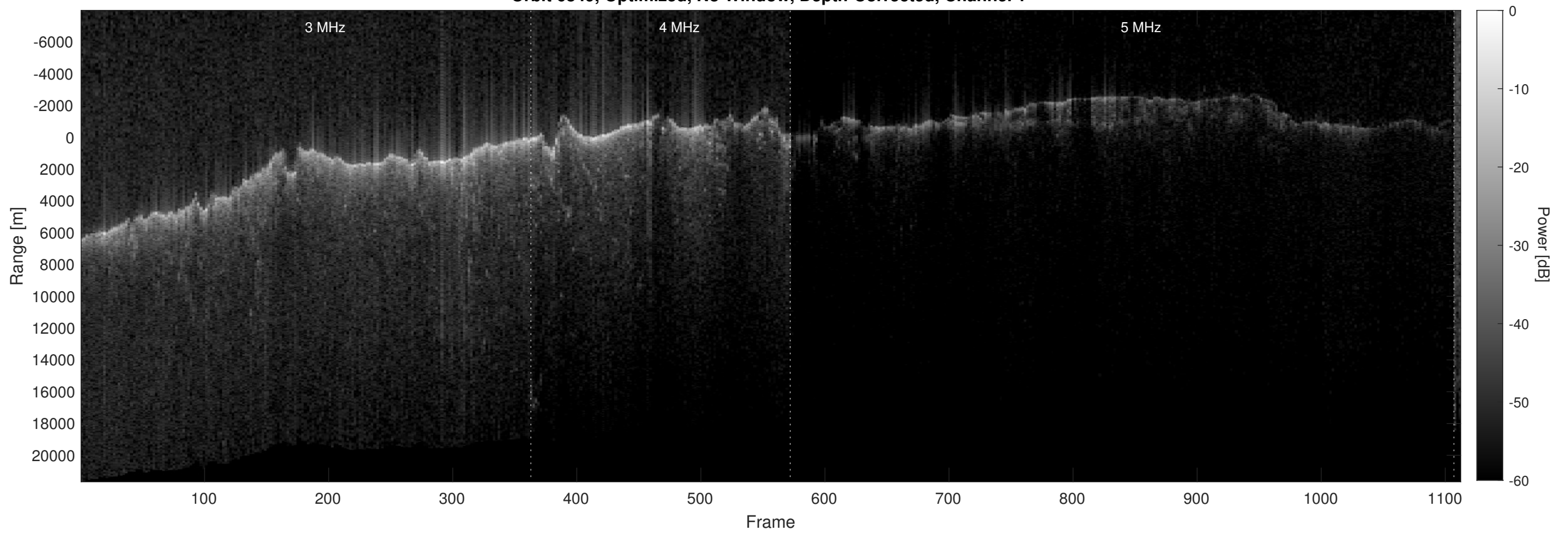
Orbit 6849, Optimized, No Window, Depth-Corrected, Channel 2
