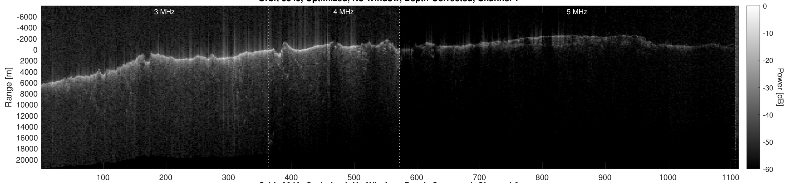
Orbit 6849, Optimized, No Window, Depth-Corrected, Channel 2
