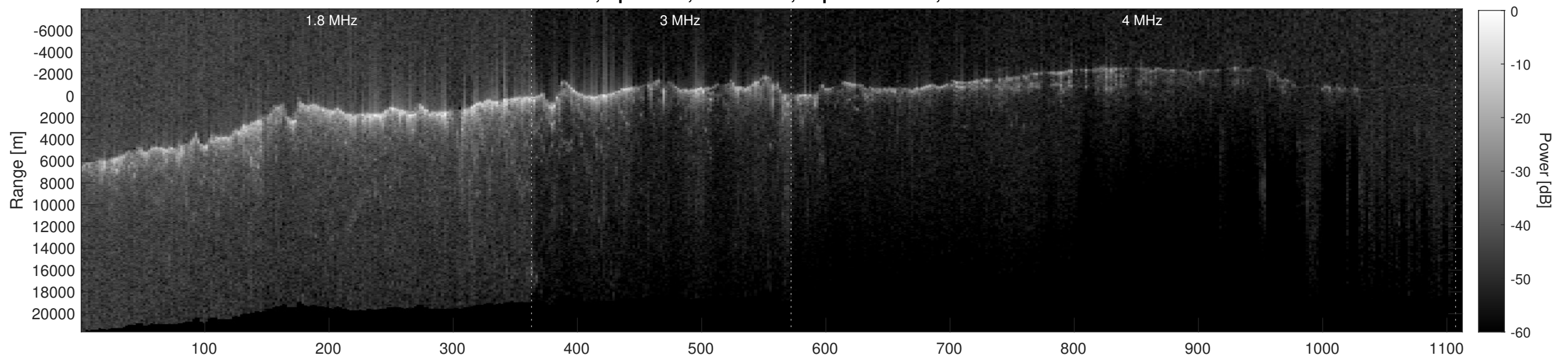
Orbit 6849, Depth-Corrected Cluttergram
