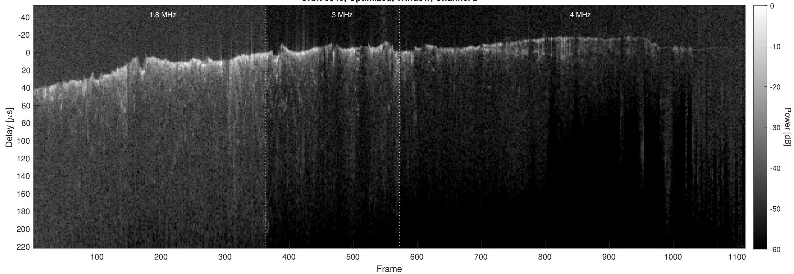
Orbit 6849, Optimized, Window, Channel 2
