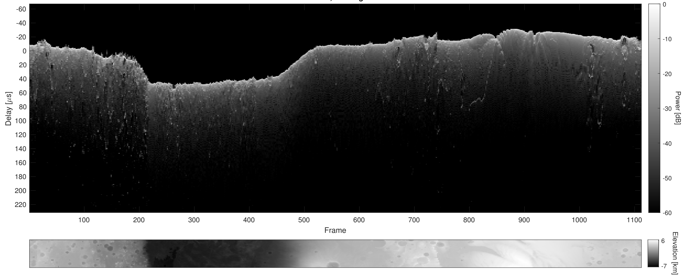
Orbit 6850, Cluttergram
