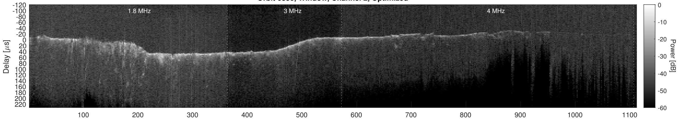
Orbit 6850, Cluttergram
