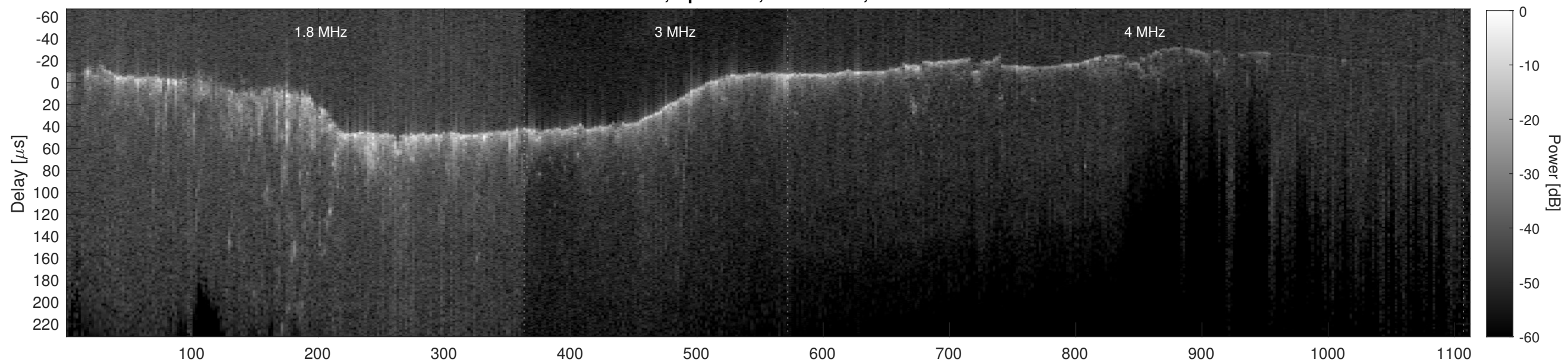
Orbit 6850, Cluttergram
