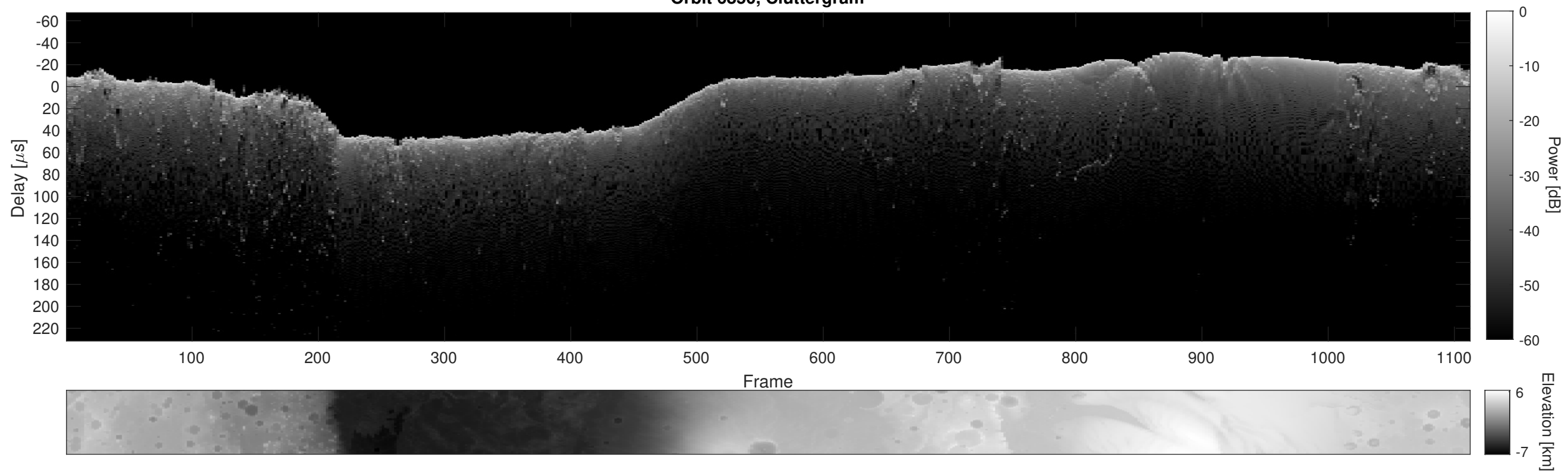
Orbit 6850, Cluttergram
