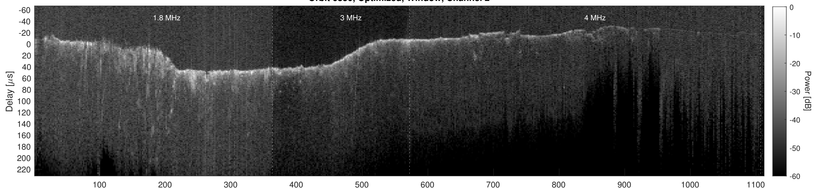
Orbit 6850, Cluttergram
