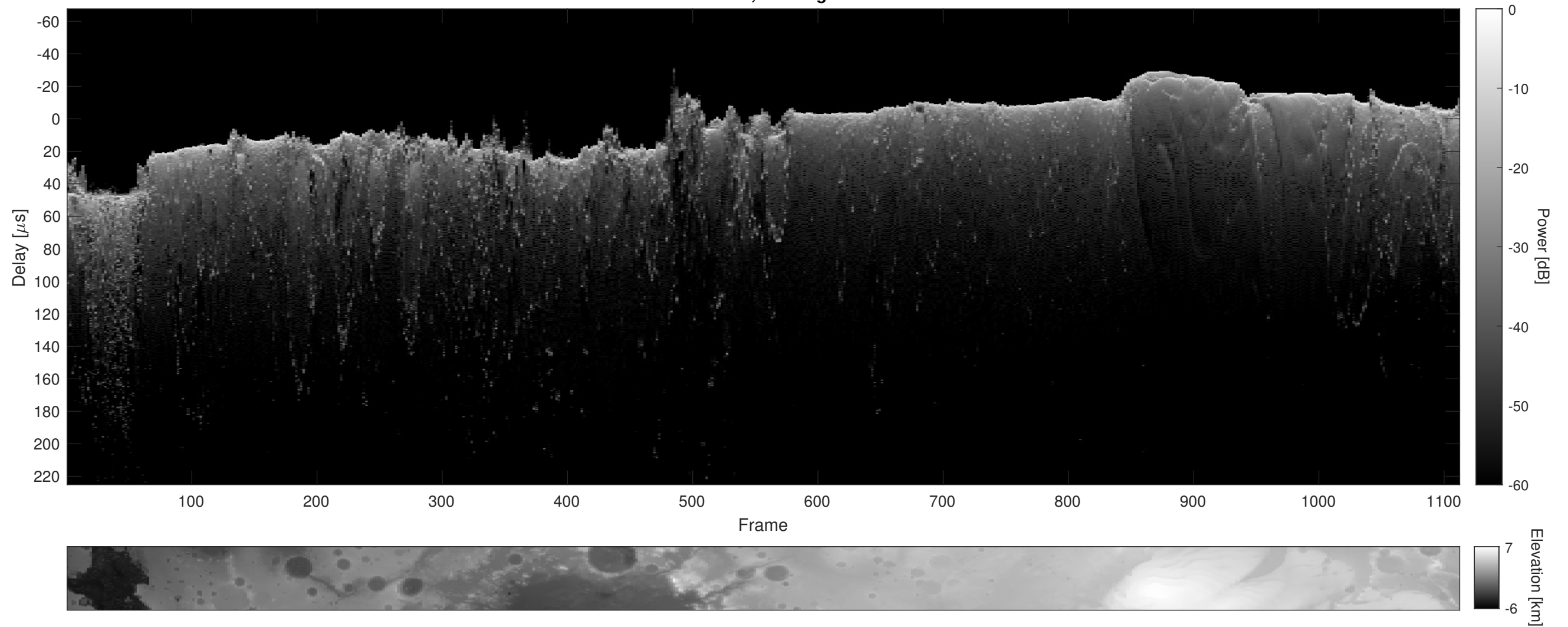
Orbit 6851, Cluttergram
