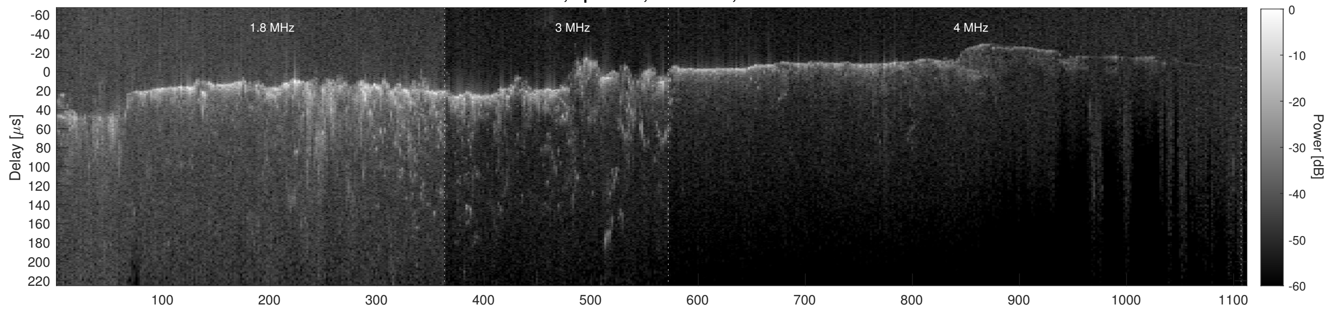
Orbit 6851, Cluttergram
