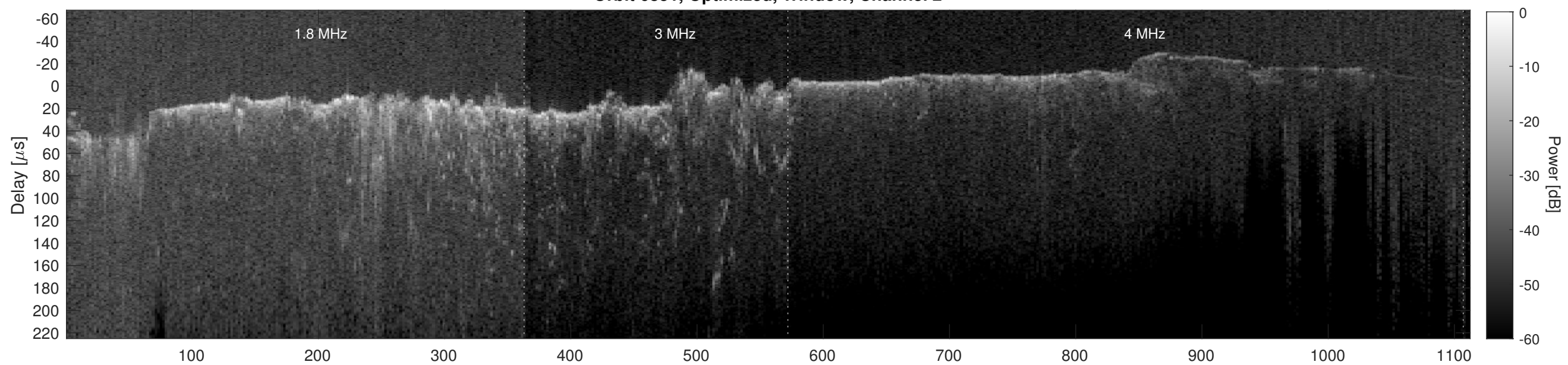
Orbit 6851, Cluttergram
