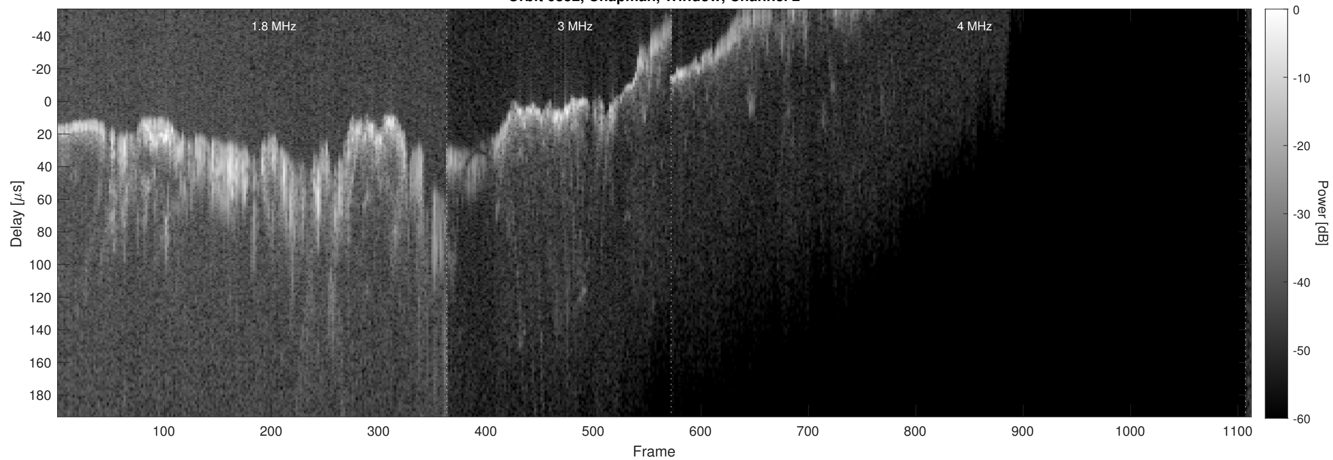
Orbit 6852, Chapman, Window, Channel 2
