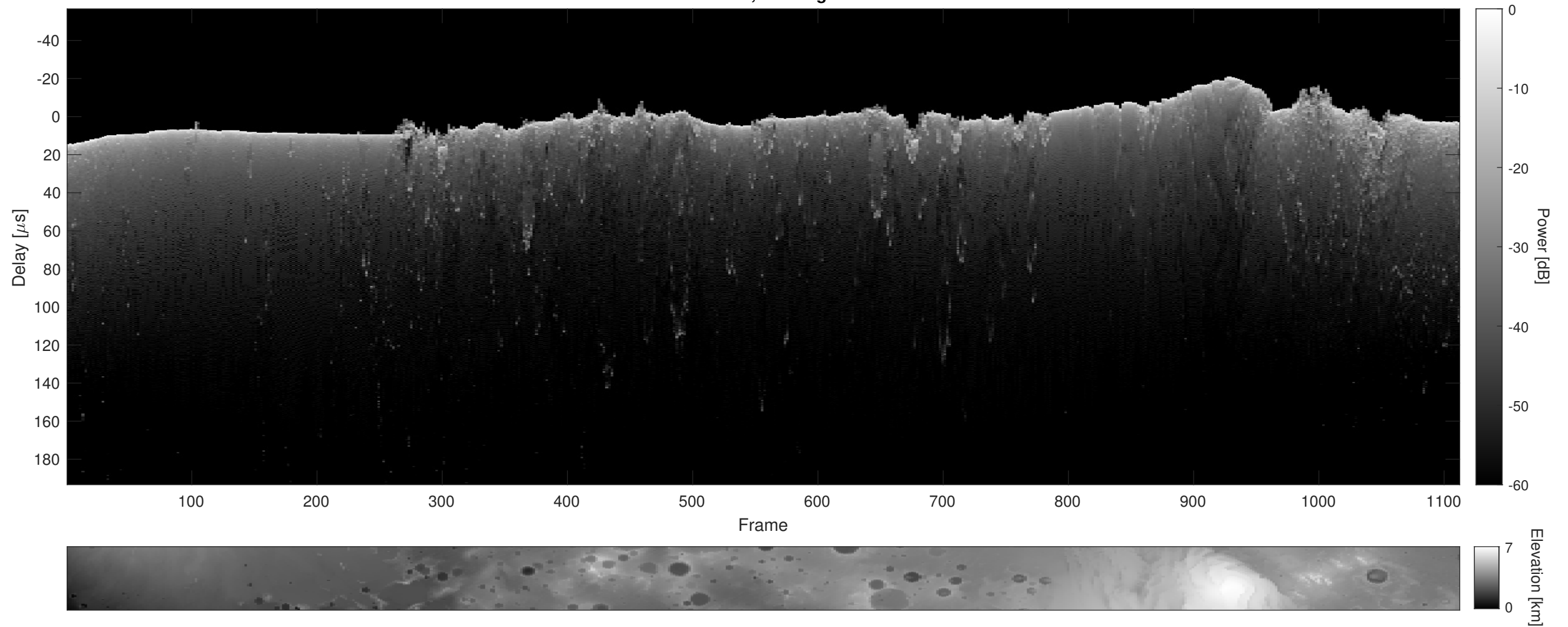
Orbit 6852, Cluttergram
