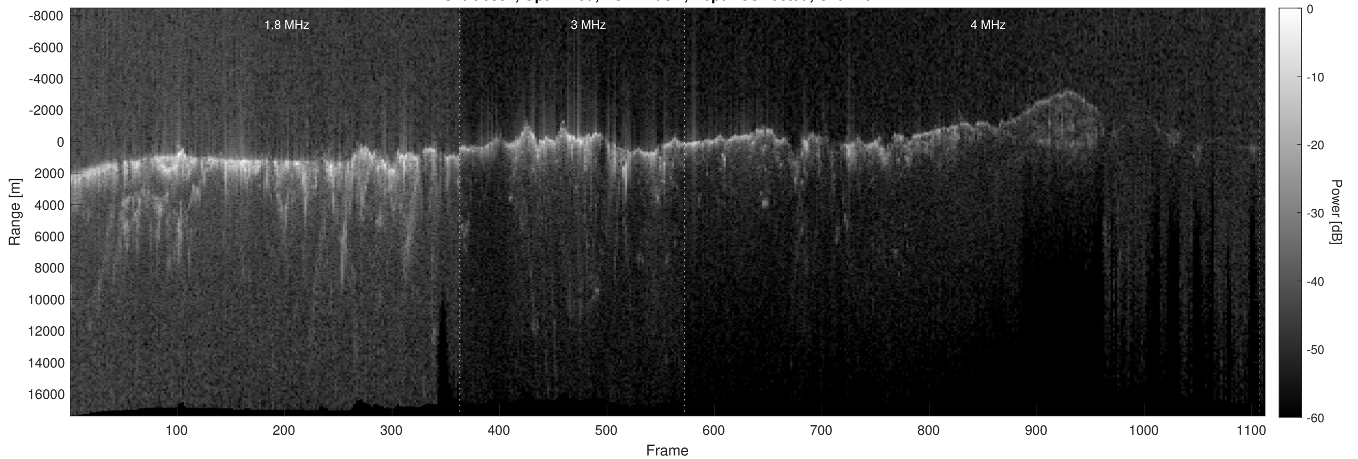
Orbit 6852, Optimized, No Window, Depth-Corrected, Channel 2
