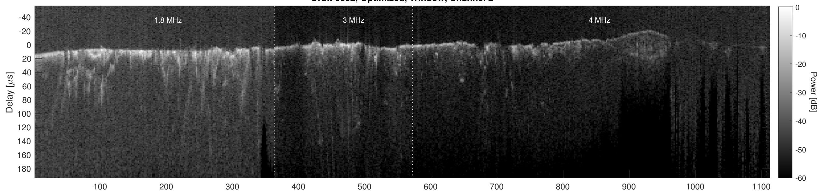
Orbit 6852, Cluttergram
